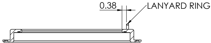
SECTION P-P
