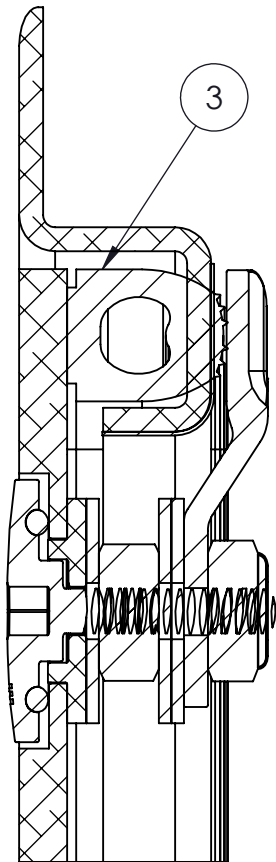
CUT THRU DOG SCALE 1:1
