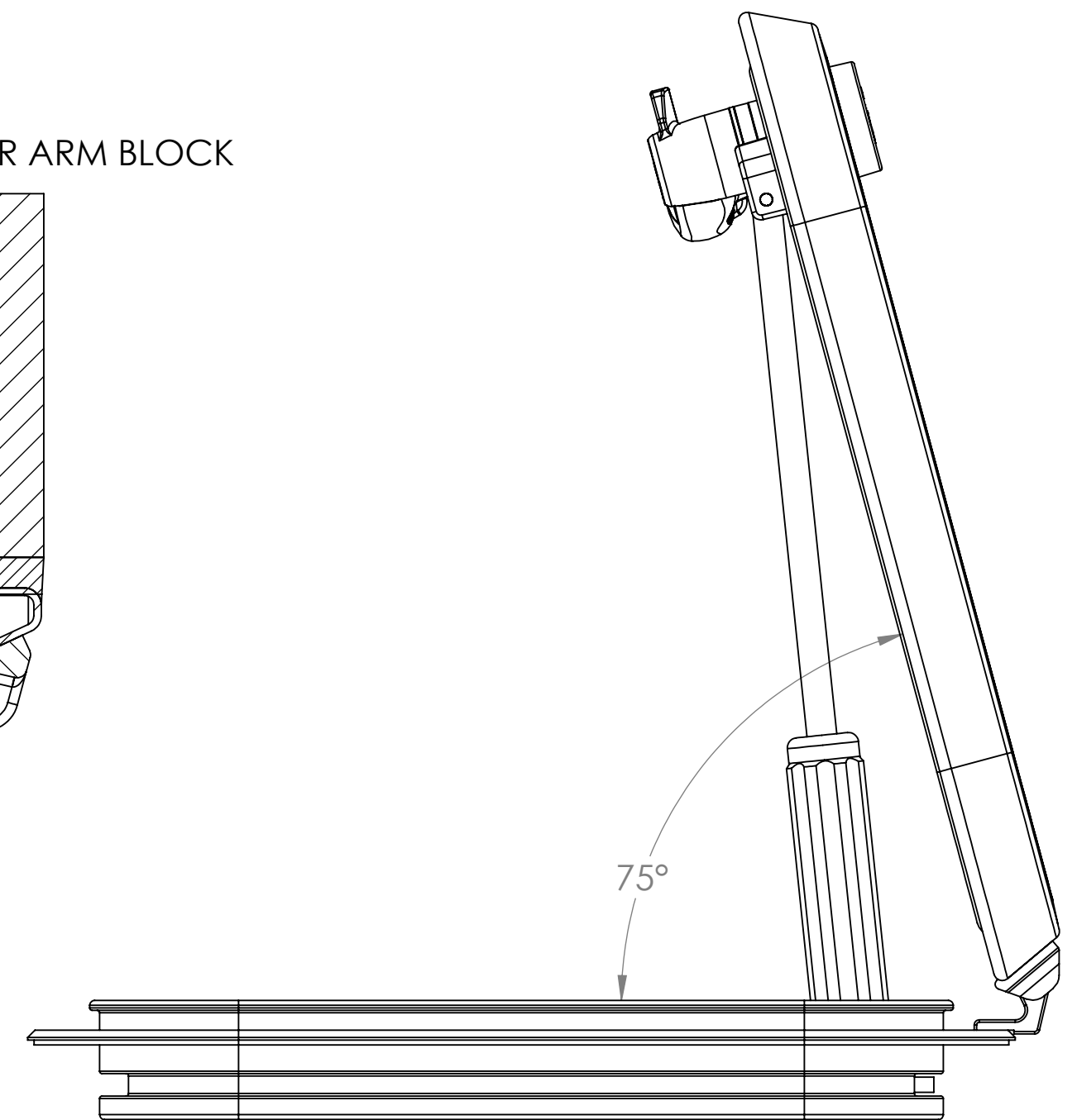
SECTION E-E SCALE 1 : 1
