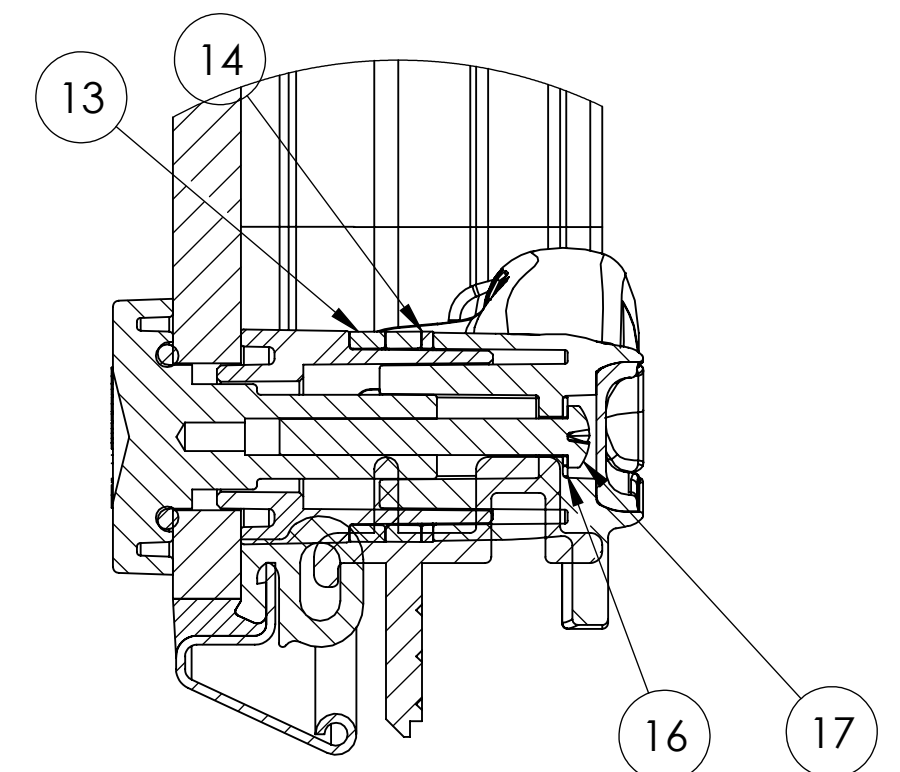
DETAIL D SCALE 1 : 1
