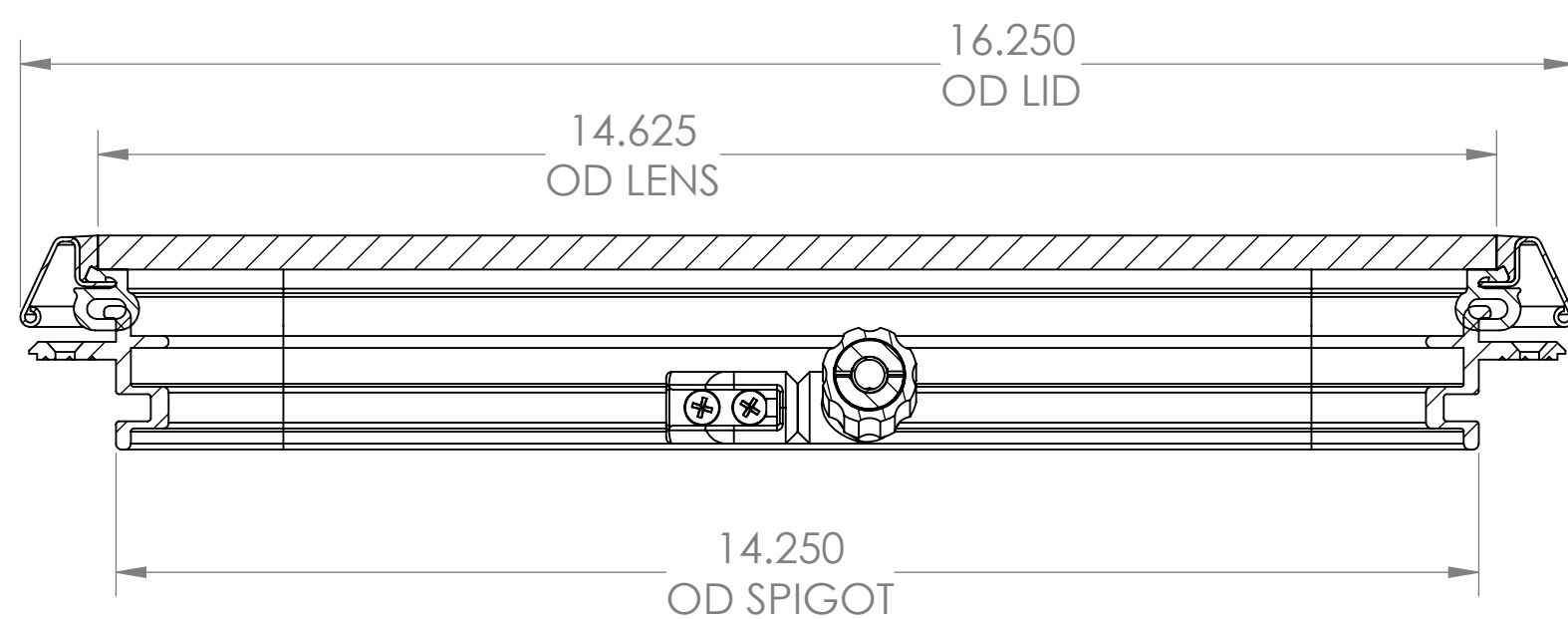
SECTION B-B
