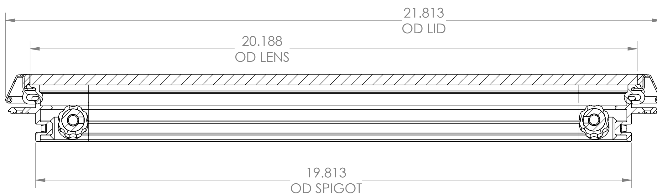
SECTION B-B
