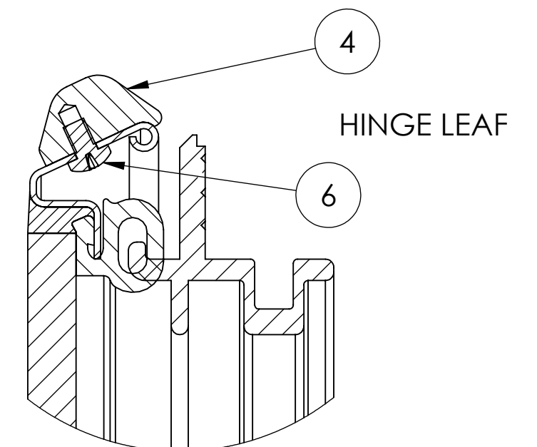
DETAIL C SCALE 1 : 1
