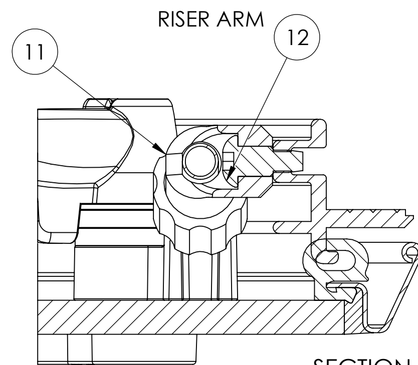
SECTION E-E SCALE 1 : 1
