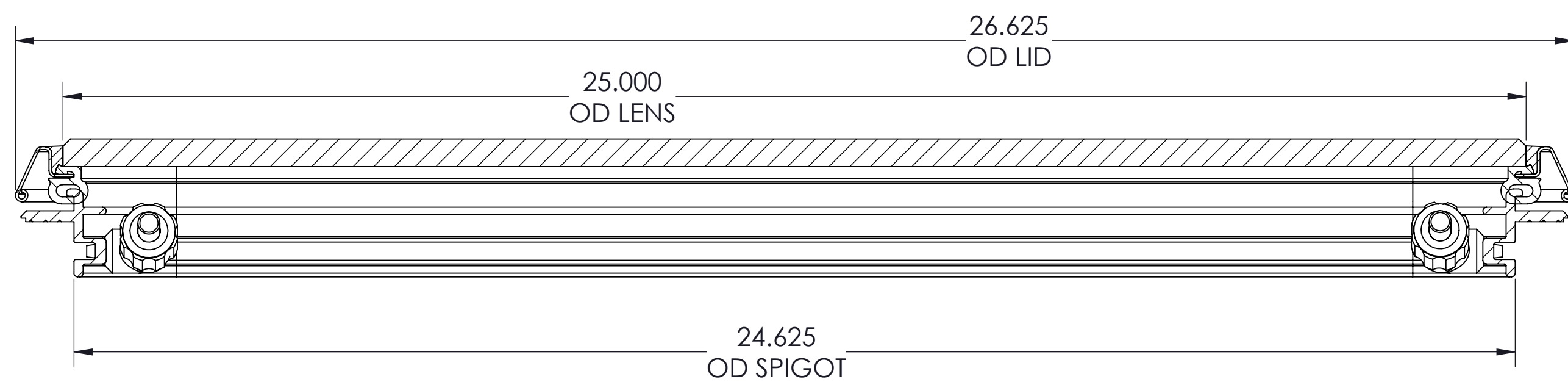
SECTION B-B
