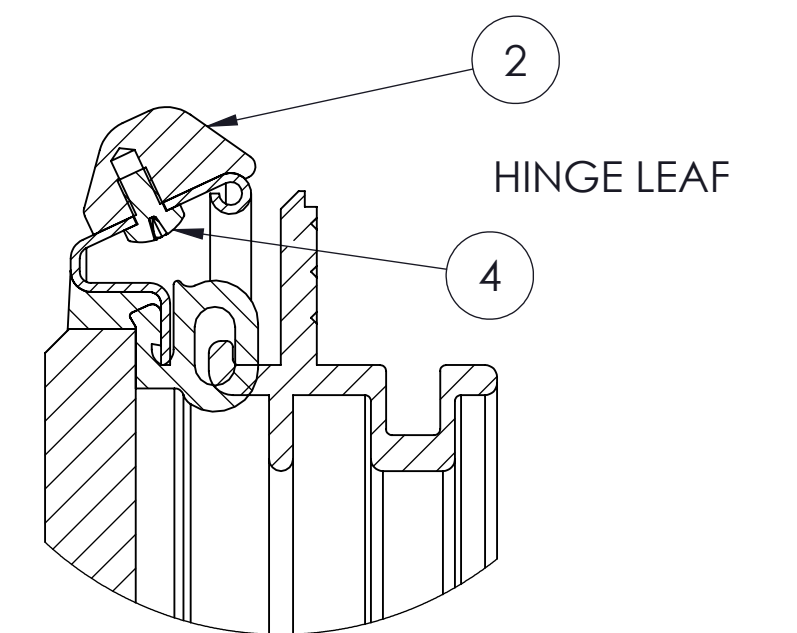
DETAIL C SCALE 1 : 1
