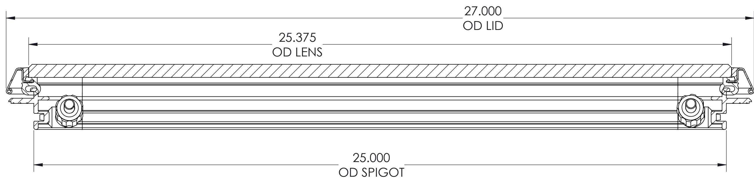
SECTION B-B
