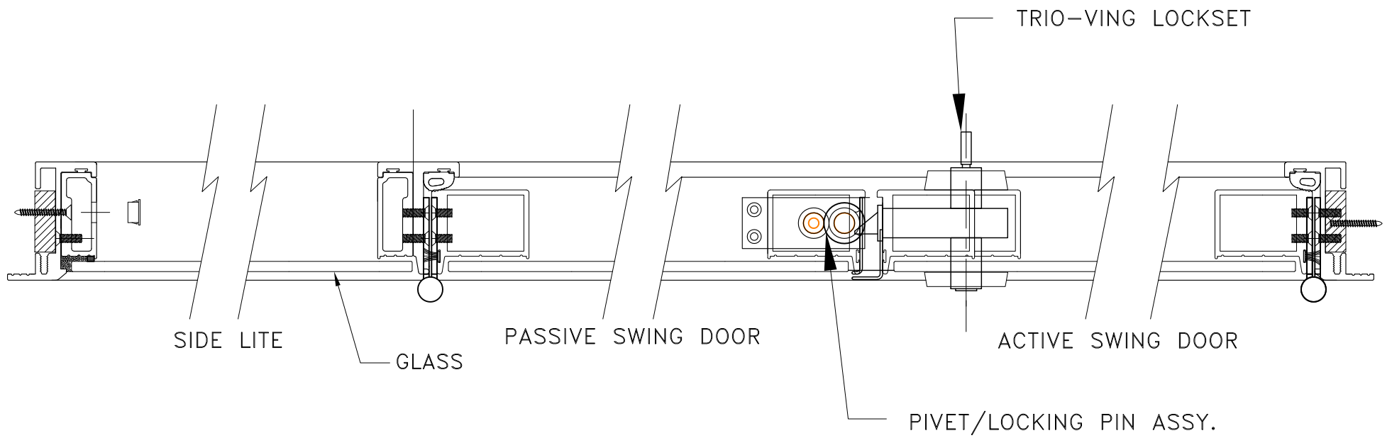
2 PANEL SWING WITH 1 SIDELITE
