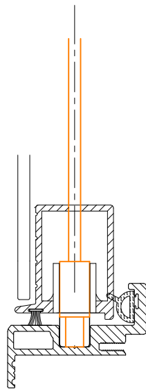
PIVET/LOCKING PIN ASSY.
