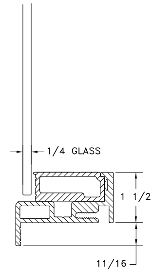
SECTION THRU SIDE LITE
