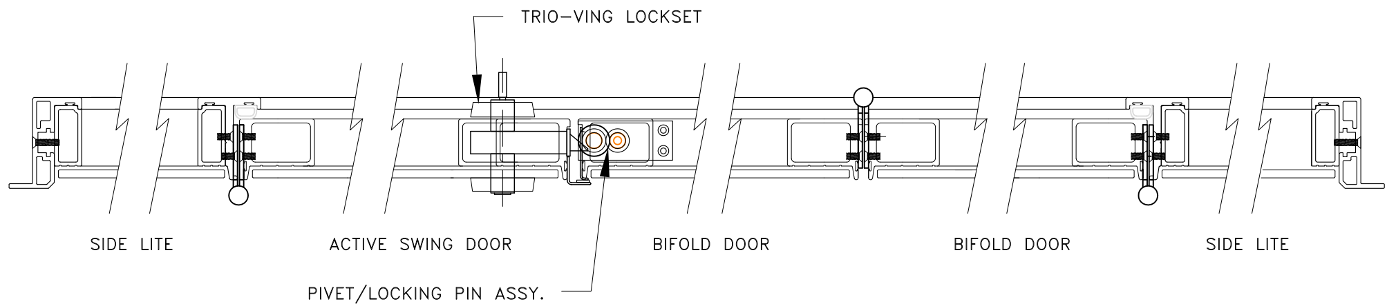
3 PANEL SWING/BIFOLD WITH 2 SIDELITE
