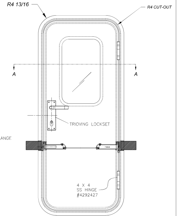
DOOR UNIT - OUTSIDE VIEW
