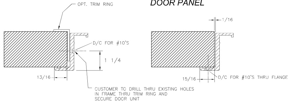
FRAME MOUNTING DT'L
