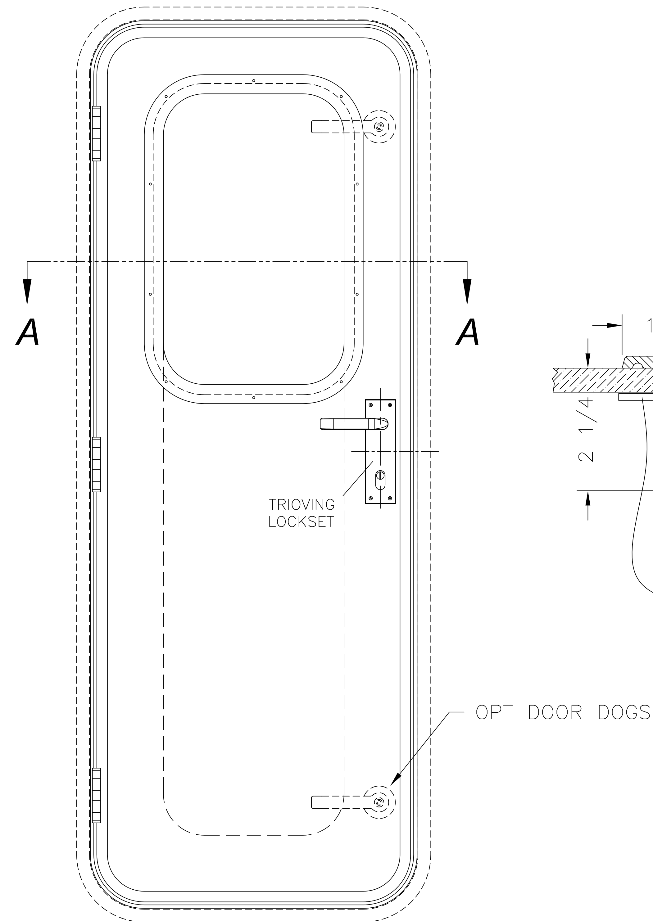
1600-RD IN-SWING DOOR - INSIDE VIEW
