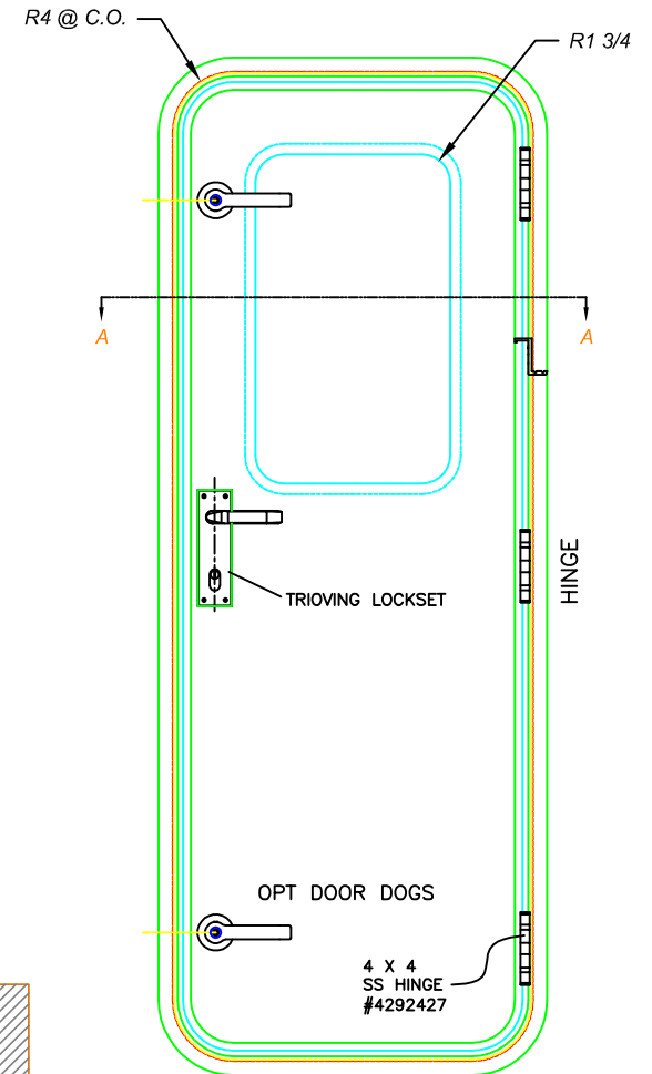
DOOR UNIT - OUTSIDE VIEW
