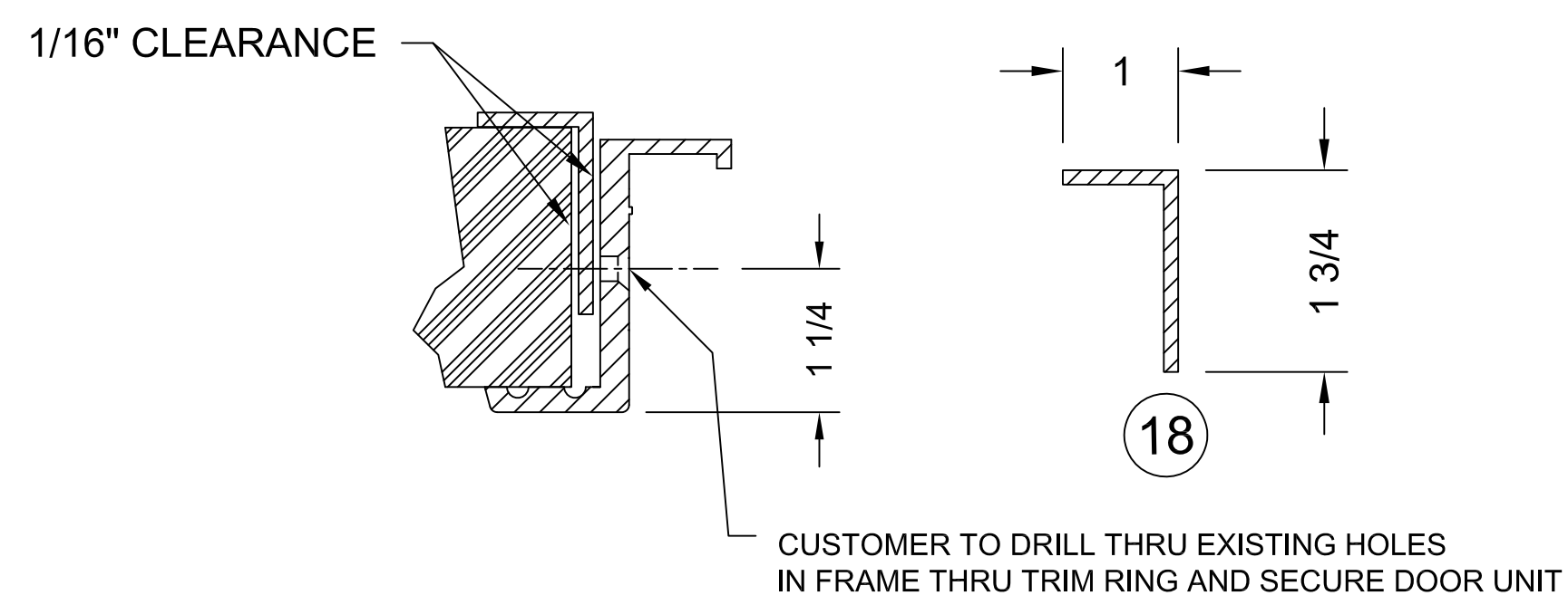
FRAME MOUNTING DT'L
