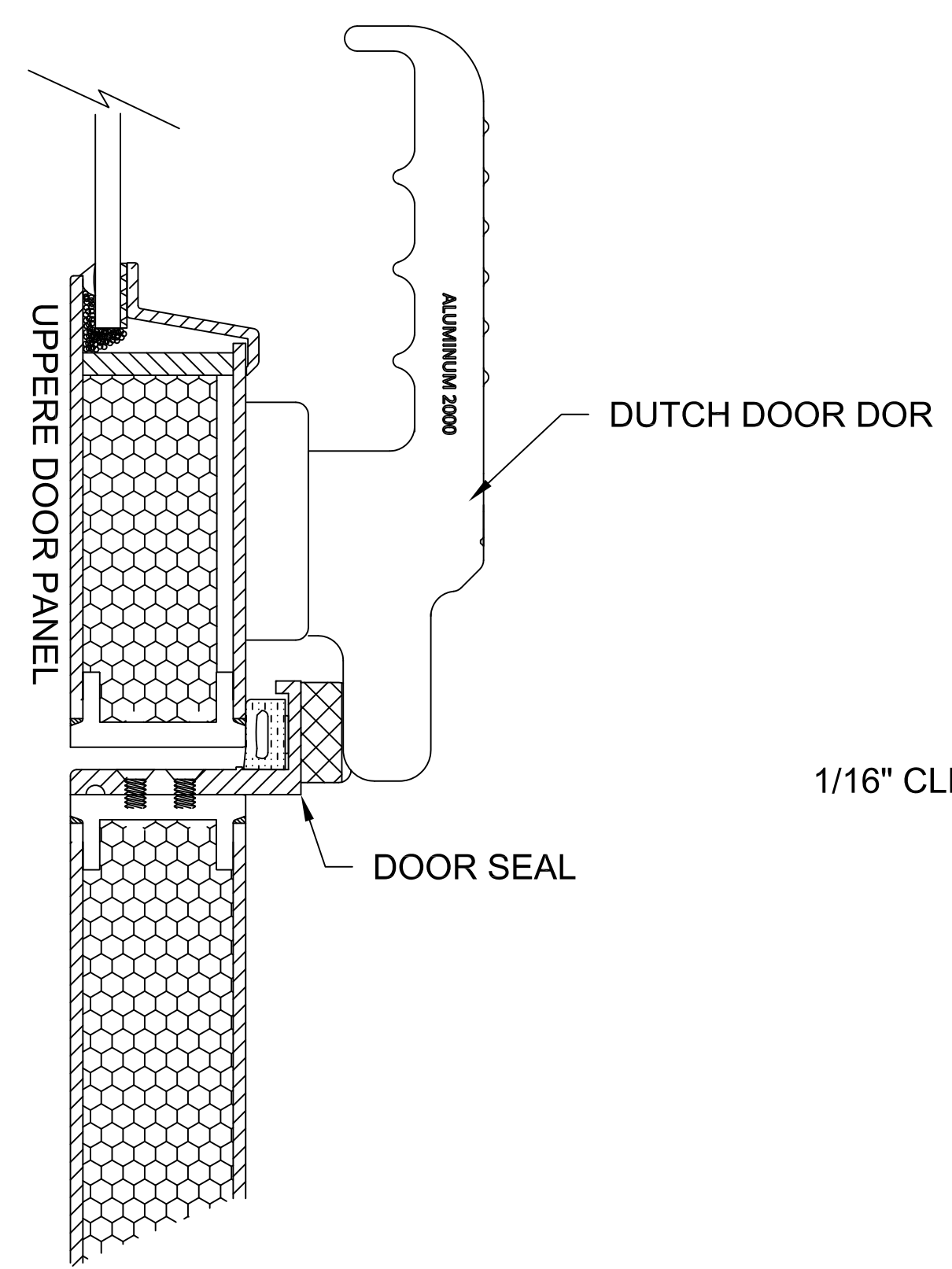
DUTCH DOOR SEAL
