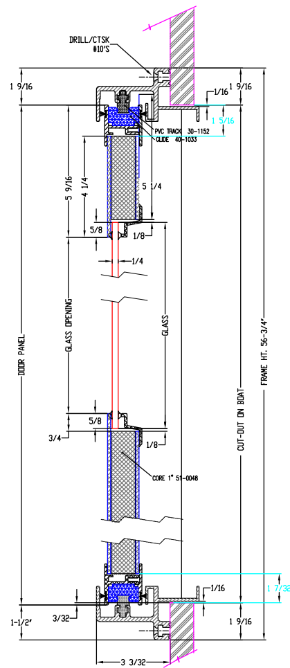
SECTION VIEW
